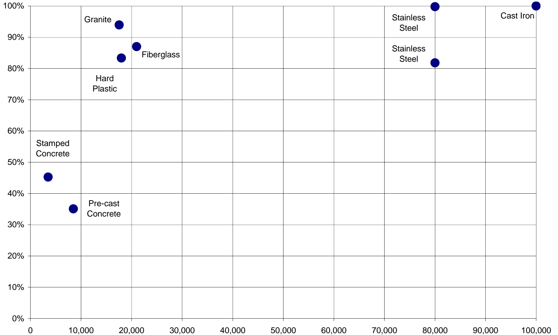
Percent of Domes Remaining after 30 snow plow passes vs. Compressive Strength
